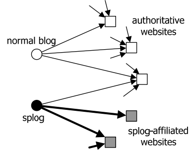
Figure 3: Normal blogs tend to link to authoritative websites while splogs frequently link to affiliate websites that are not authorities. The thickness of the arrow from the splog indicates the frequency with which the splog links to a non-authoritative, affiliate website.
