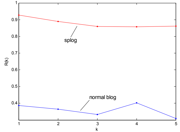
Figure 1: The figure shows the difference in the autocorrelation function between a splog and a normal blog. Notice that auto-correlation function for a splog is very high and nearly constant, while the values for a normal blog are relatively low and fluctuate. These graphs have been derived from a splog and a normal blog from the TREC dataset.
