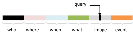
Figure 5: The query vector \mathbf{q} has six facets. The query can be along any of the six facets. Typically, we would query for an image, and the iterative process would retrieve top ranked annotations for the other five facets.
